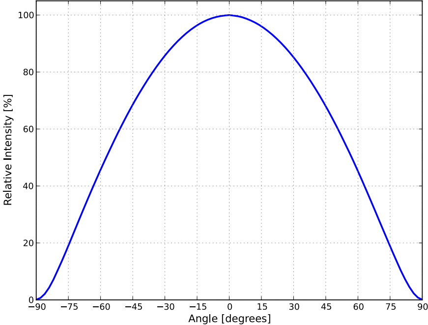
Figure 5. Typical radiation pattern for LUXEON CoB Core Range PW at specified test current, T_j=85^{\circ}\text{C} .
